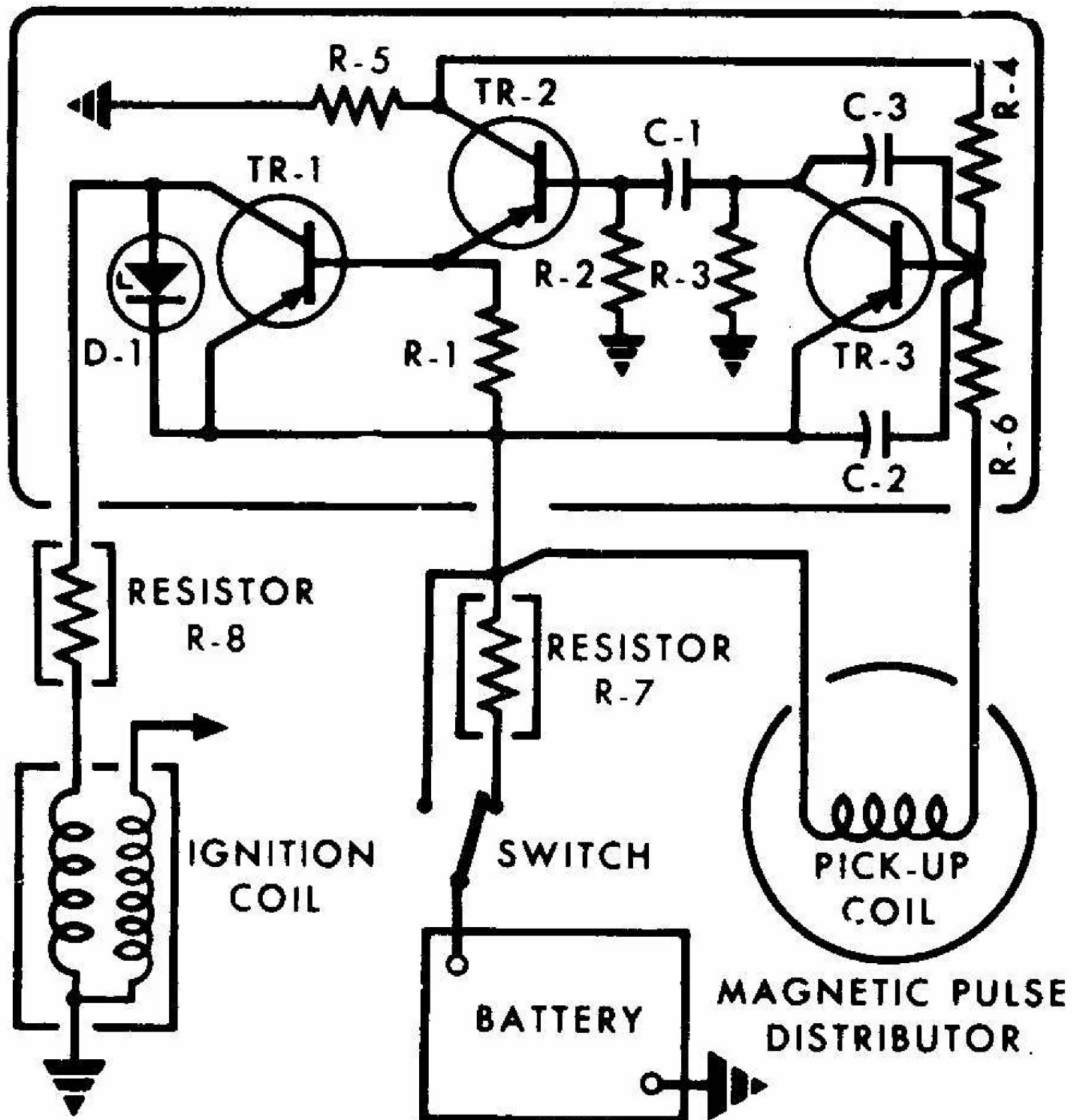
TRANSISTOR IGNITION AMPLIFIER CIRCUIT
