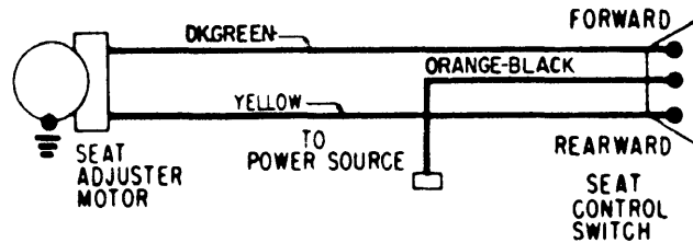
GENERAL MOTORS 2-WAY POWER SEAT WIRING
