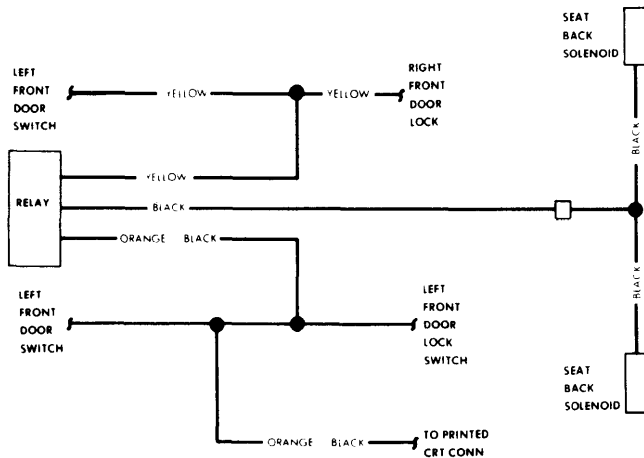
GENERAL MOTORS SEAT BACK LATCH WIRING
