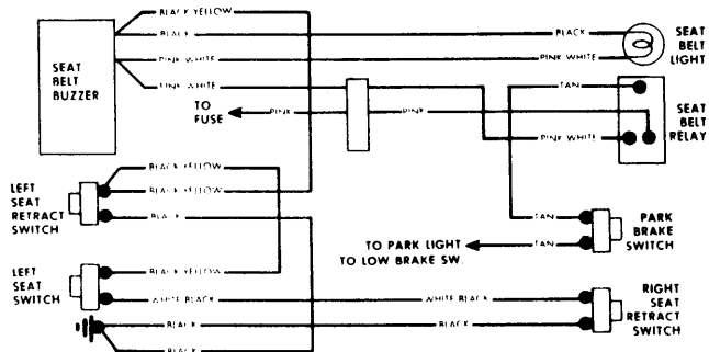
CORVETTE SEAT BELT WARNING SYSTEM
