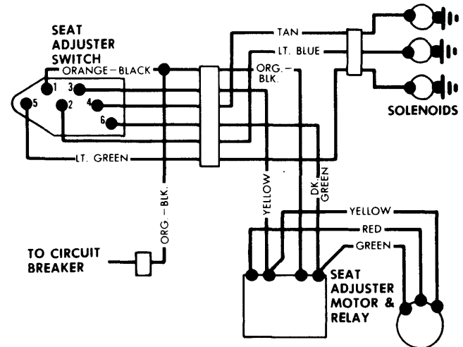
GENERAL MOTORS 6-WAY POWER SEAT WIRING
