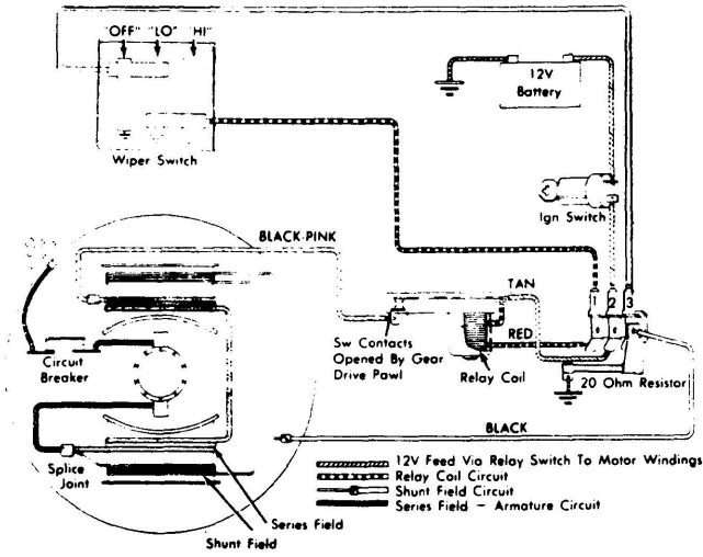
GENERAL MOTORS ROUND-MOTOR WIPER SYSTEM WIRING
