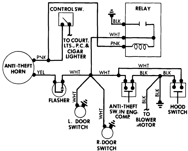
Chevrolet Corvette Anti-Theft Alarm System Wiring Diagram
