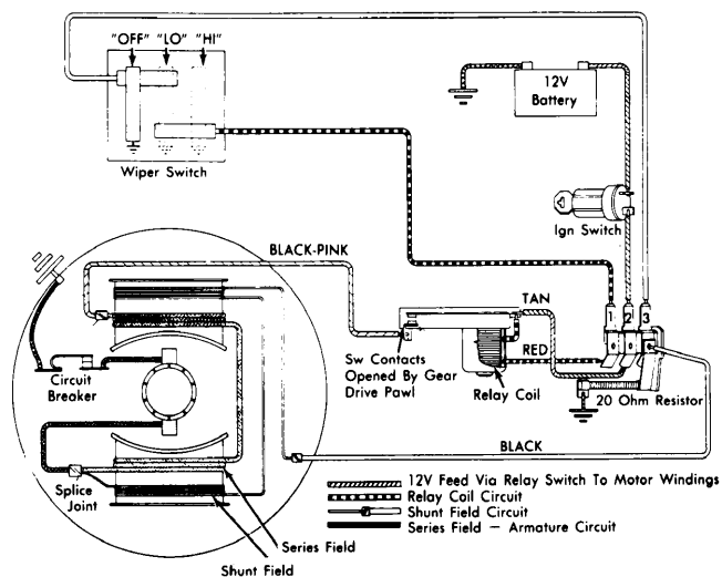
General Motors Round Motor Wiper System Wiring Diagram
