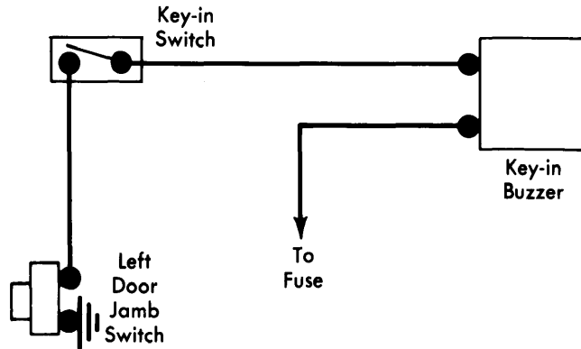
General Motors Separate Key Warning Buzzer Wiring Diagram Chevrolet
