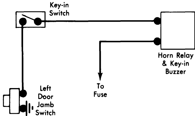
General Motors Key Warning Buzzer in Horn Relay Wiring Diagram
