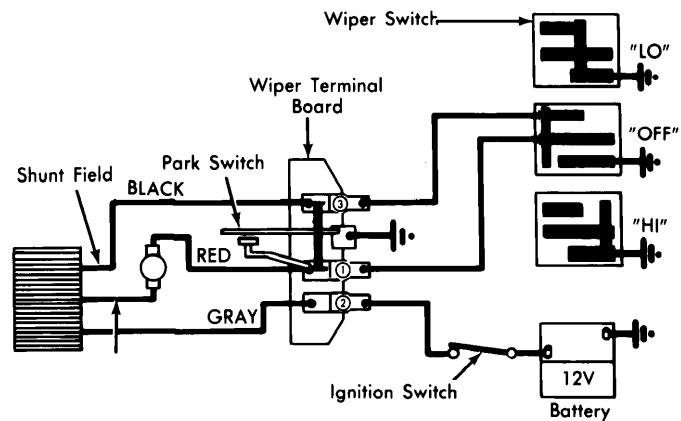
General Motors Square Motor Wiper System Wiring Diagram
